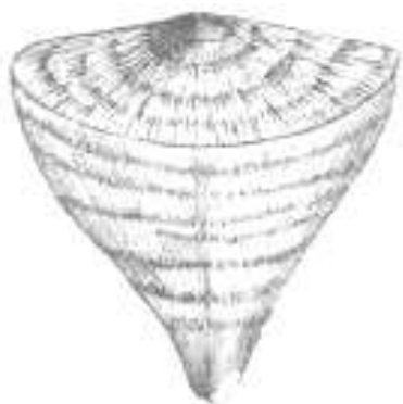
Calceola sandalina
